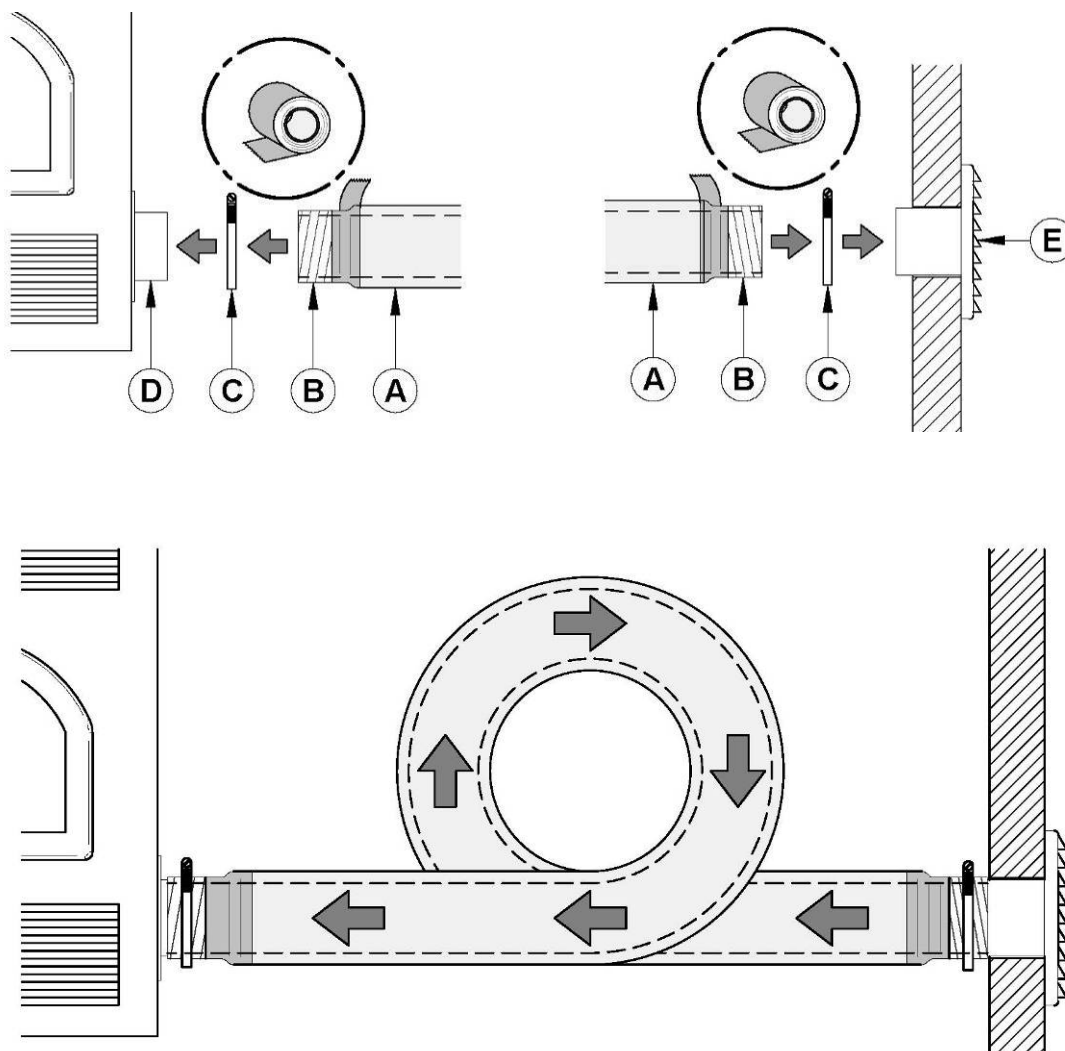
Fresh air intake kit (J) installation
